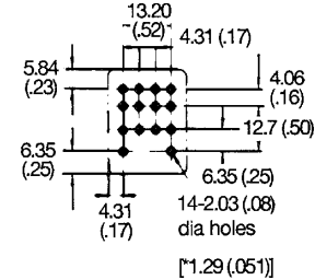
4PDT
